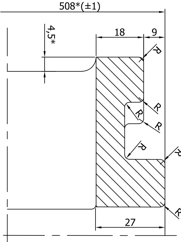
B-B (1:1)
